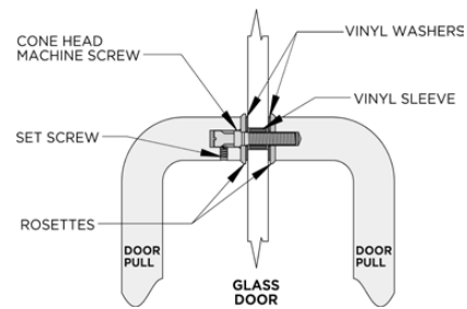
#5G = BACK TO BACK MOUNTING FOR GLASS DOORS
