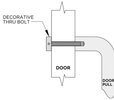
#4 = SINGLE DECORATIVE MOUNTING FOR WOOD AND METAL DOORS
