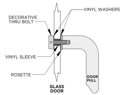
#4G = SINGLE DECORATIVE MOUNTING FOR GLASS DOORS
